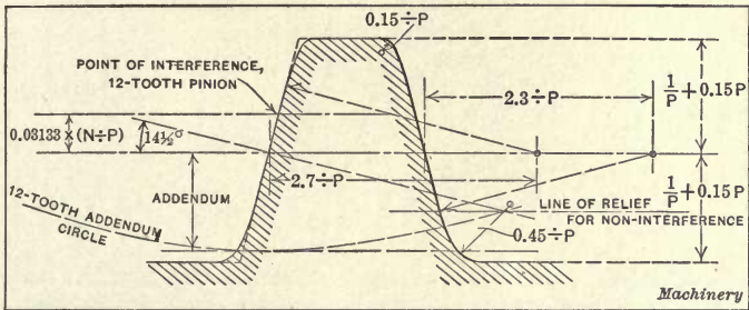
Fig. 2. Hob Tooth designed to generate the Approximate Shape of a 14½-degree Involute Milled Tooth
