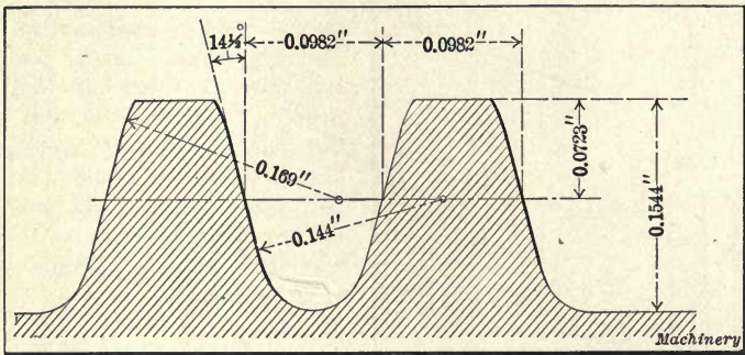
Fig. 6. Special Hob Tooth Dimensions
